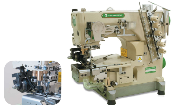
MJ2600D-356/MR/HG/VDA/EWT(AWT)/BT With left hand side fabric trimmer (MR), and belt-drive top feeder (BT) 附左切刀修布邊裝置(MR)、及皮帶式上送裝置(BT)
